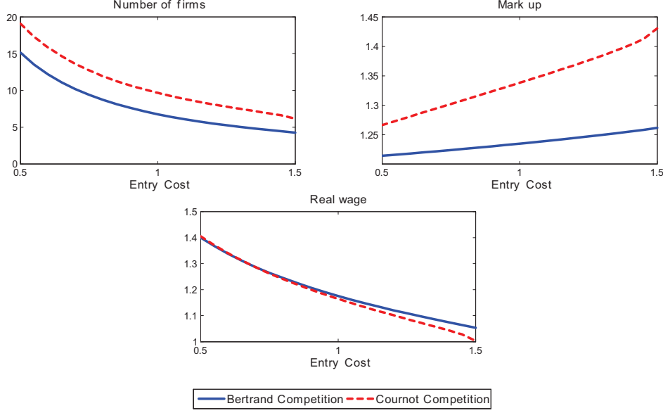
Figure 1: Steady state value of some selected variables as a function of the entry cost \psi .
