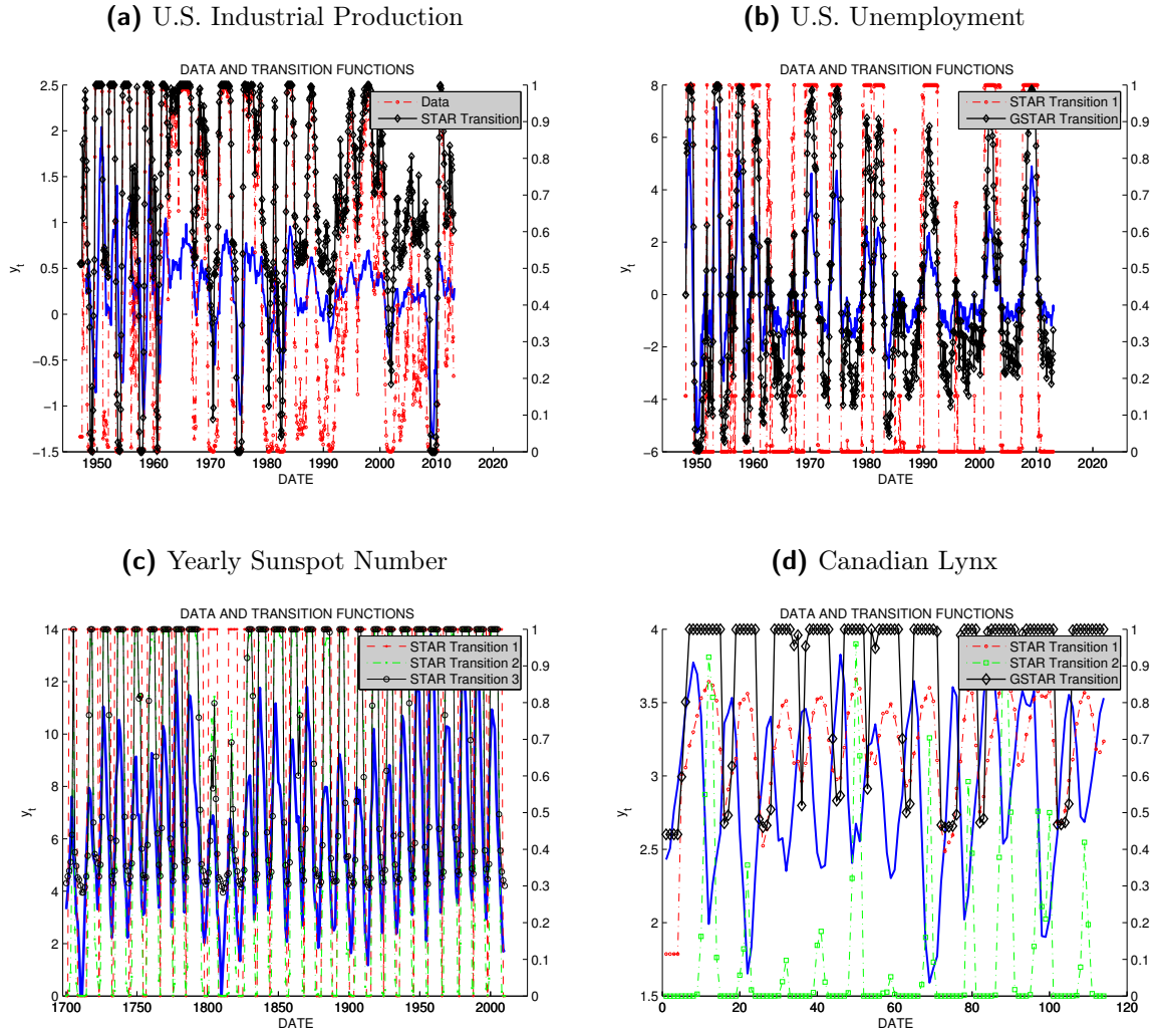
Figure 5: Estimated transition function for (MR)STAR and GSTAR specifications.
